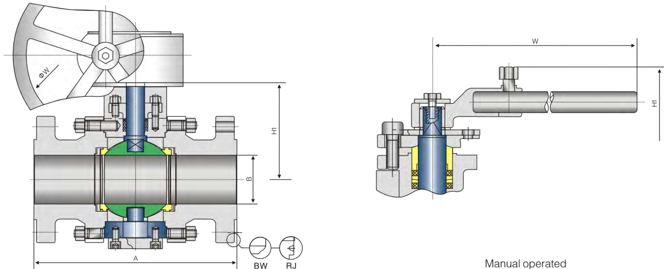
Manual operated
