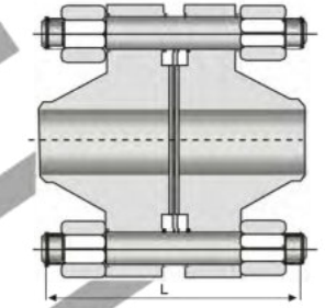
ANSI Class600Lb/900Lb 0.25"(6.4mm) Raised face joint
